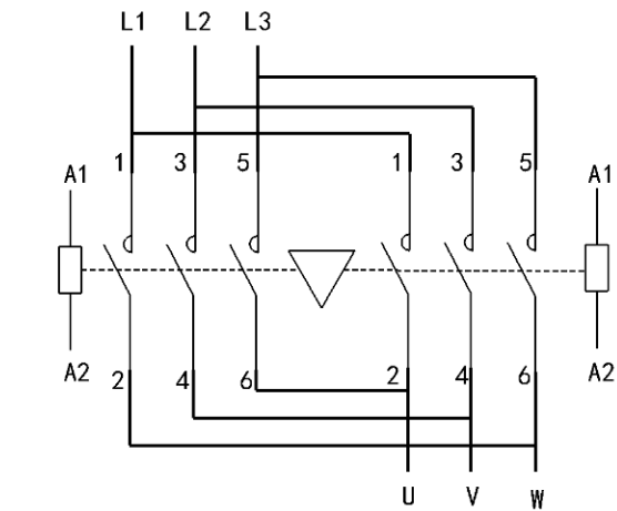
Wiring Diagram of Motor-controlled Power Reversible Contactor
