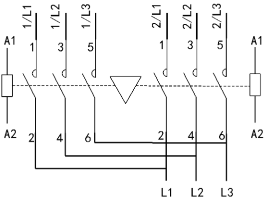
Wiring Diagram of Distribution Conversion
